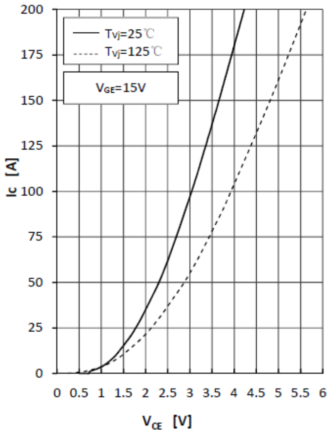
Fig1.IGBT Output Characteristics
