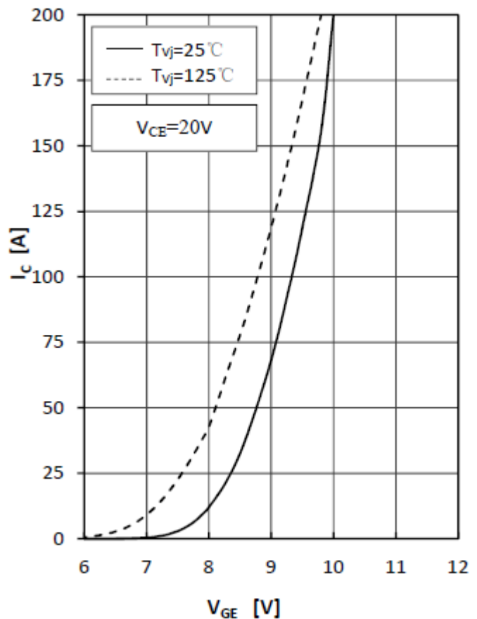
Fig2.IGBT Transfer Characteristics
